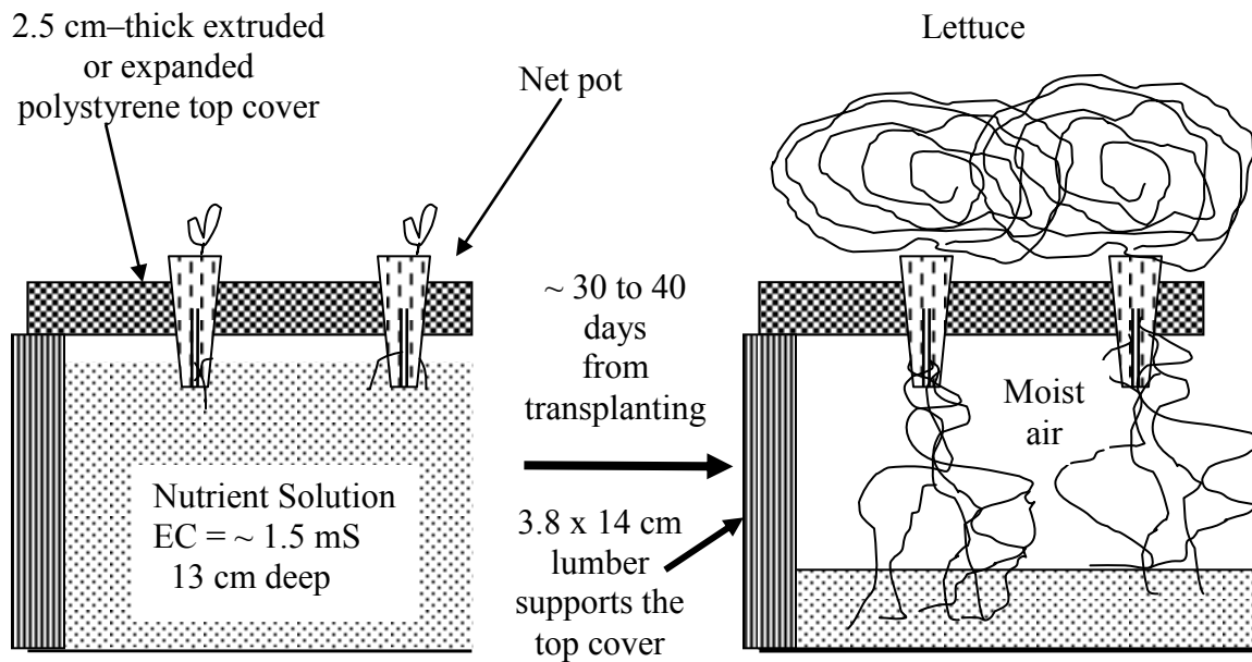
Fig. 3. Growing lettuce by a non-circulating hydroponic system where the top cover is supported by the tank frame.
